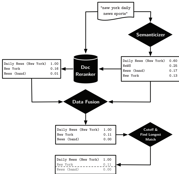
Figure 1: A schematic view of our system pipeline. A query is given as input to the Semantizer for generating a ranked list of candidate entities using several methods. The candidate list is refined using a document re-ranker and then all ranked lists are merged together using late data fusion. The final entities for the query are selected using cutoff on their retrieval score, and longest matches are preferred over shorter ones.
